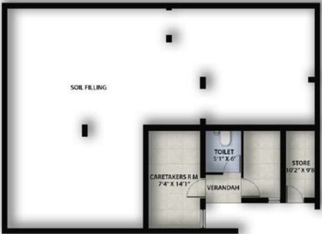
VILLA TYPE-3 (NO. 13 TO 16) STILT FLOOR
