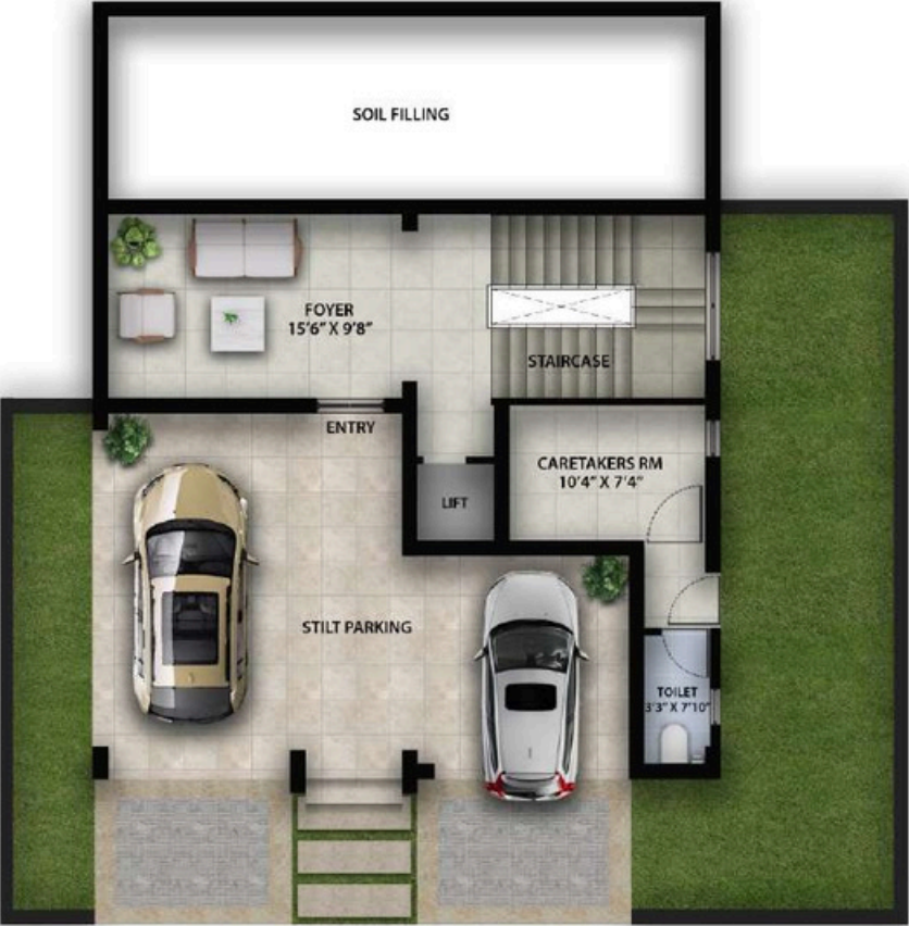
VILLA TYPE-1 (NO. 1 TO 6) STILT FLOOR
